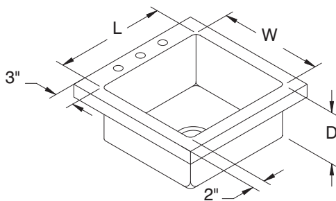
Inside Sink Bowl Dimensions
