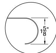
Bull Nose Edge Detail (On Front Only)
